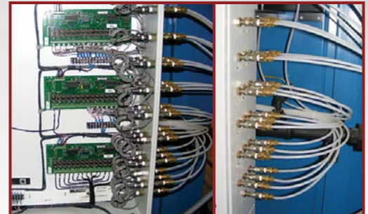
Pressure Transducer Monitoring Lines and Data Acquisition Control System
